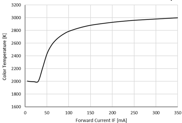
Forward Current vs. Color Temperature
